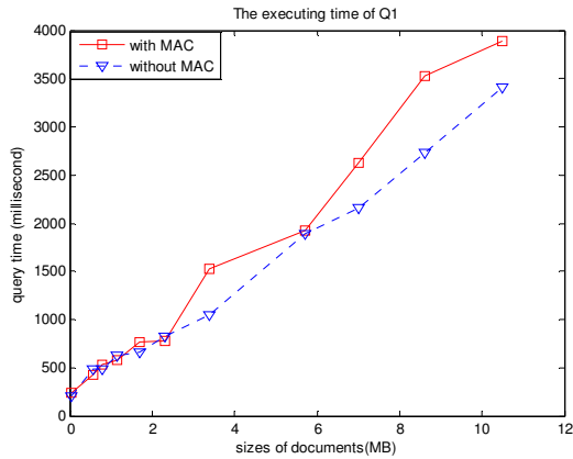
Fig.7 The executing time of Q1
